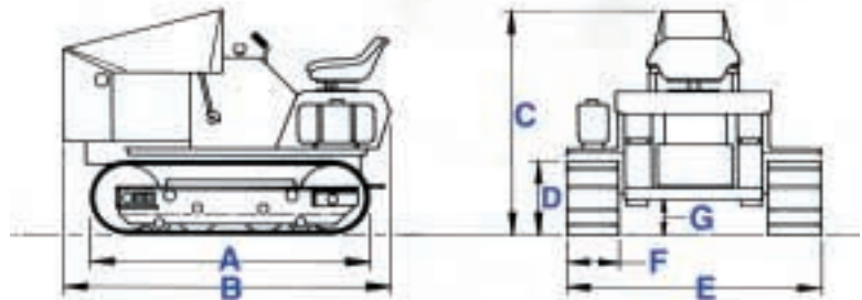
A 55-7/8" B 60" C 43-3/4" D 15-1/8" E 48-7/8" F 9-1/2" G 6"
